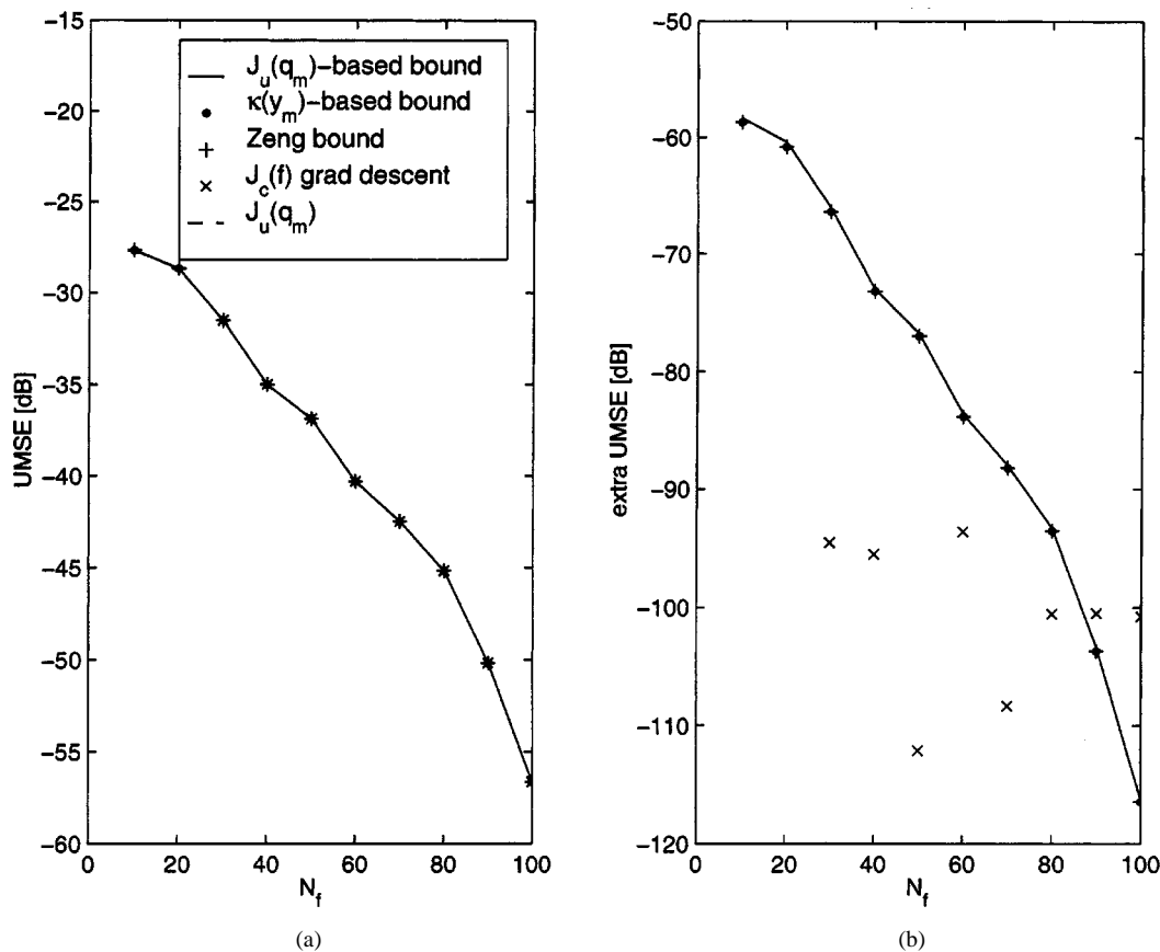
Fig. 4. Bounds on CM-UMSE versus estimator length N_f for SPIB microwave channel #5 and 8-PAM.
