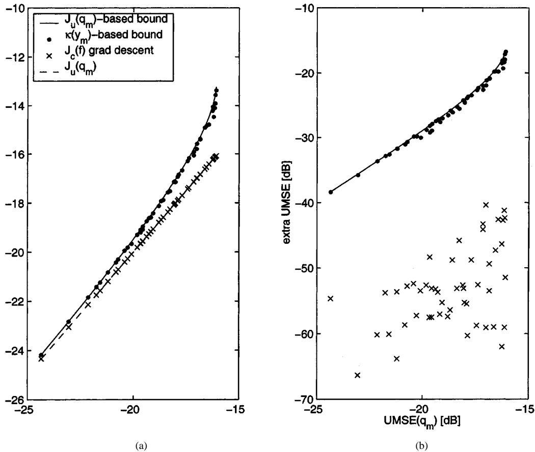
Fig. 7. Bounds on CM-UMSE for N_f = 8, 5 BPSK sources, #5 sources with \kappa_s^{(k)} = 2.9 (one of which is desired), AWGN at -30 dB, and random \mathcal{H} .
