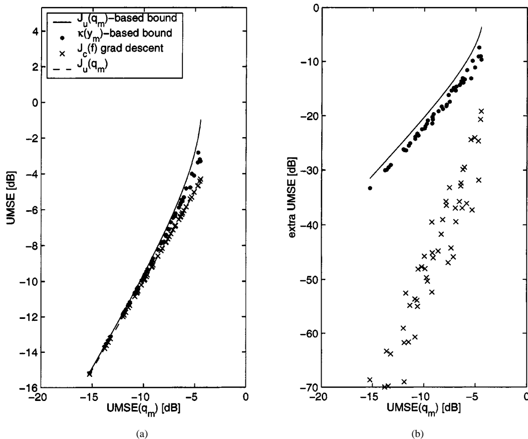
Fig. 8. Bounds on CM-UMSE for N_f = 8 , five BPSK sources (one of which is desired), #5 sources with \kappa_s^{(k)} = 4 , AWGN at -20 dB, and random \mathcal{H} .
