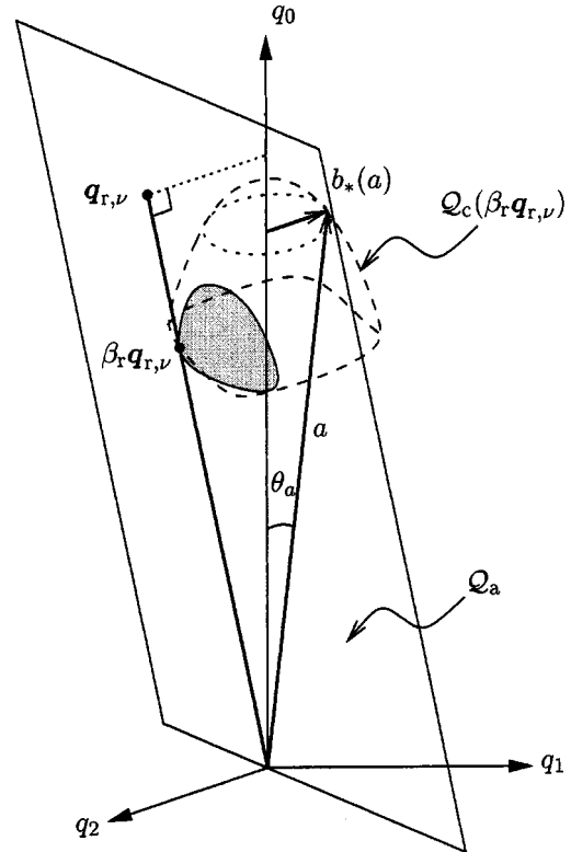
Fig. 2. Illustration of CM-UMSE upper-bounding technique using reference \mathbf{q}_{r,\nu} .
