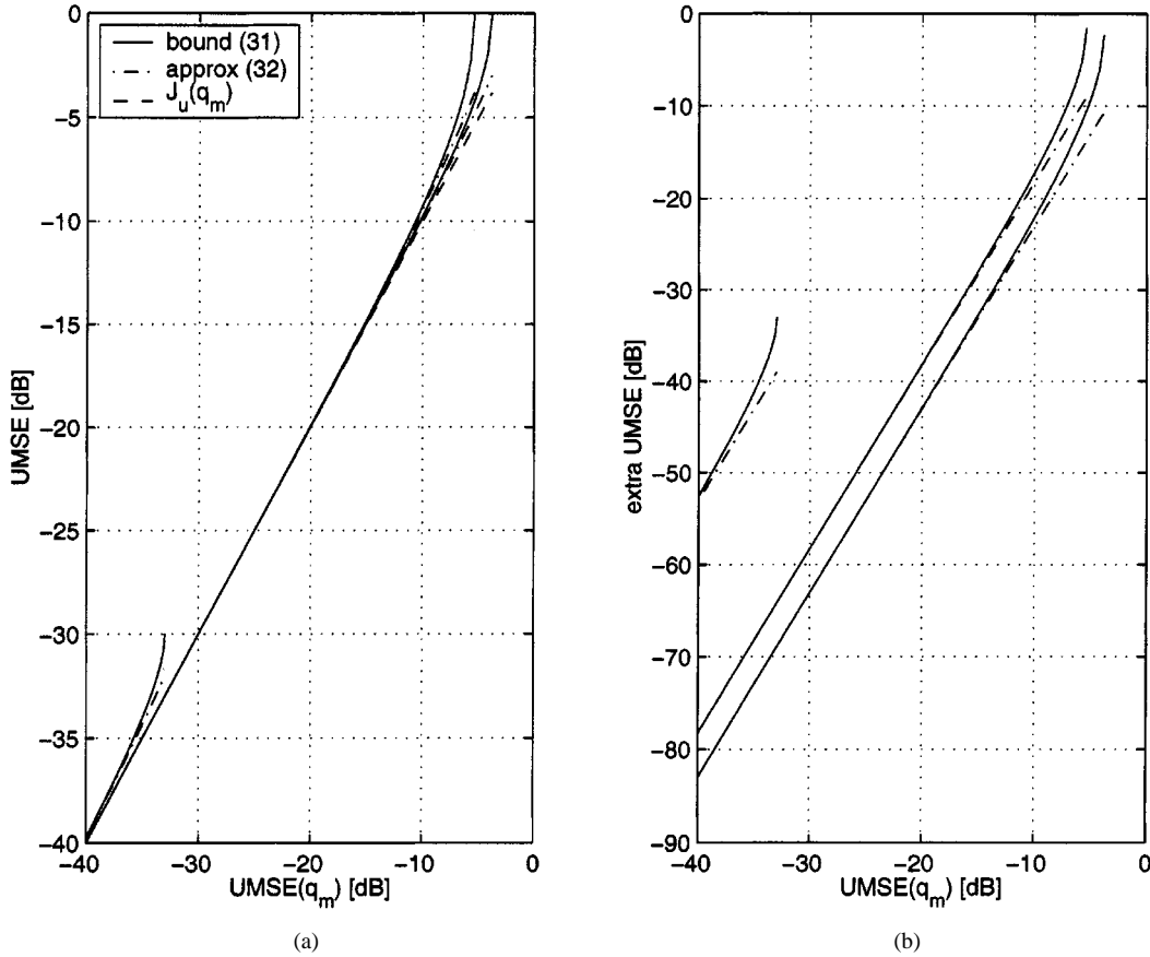
Fig. 3. Upper bound on (a) CM-UMSE and (b) extra CM-UMSE versus J_{u,\nu}(\mathbf{q}_{m,\nu}) (when \sigma_s^2 = 1 ) from (31) with second-order approximation from (32). From left to right, \{\rho_{\min}, \rho_{\max}\} = \{1000, 0\} , \{1, -2\} , and \{1, 0\} .
