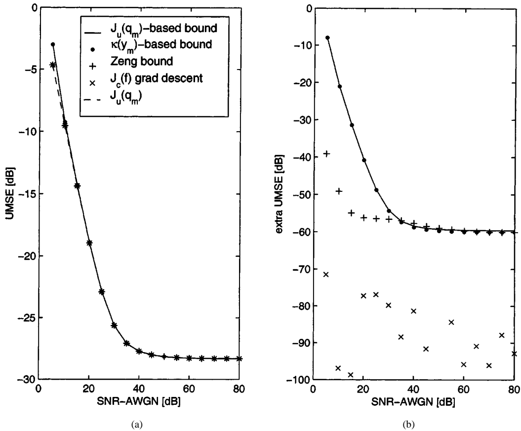
Fig. 5. Bounds on CM-UMSE versus SNR of AWGN for SPIB microwave channel #5, N_f = 20 , and 8-PAM.
