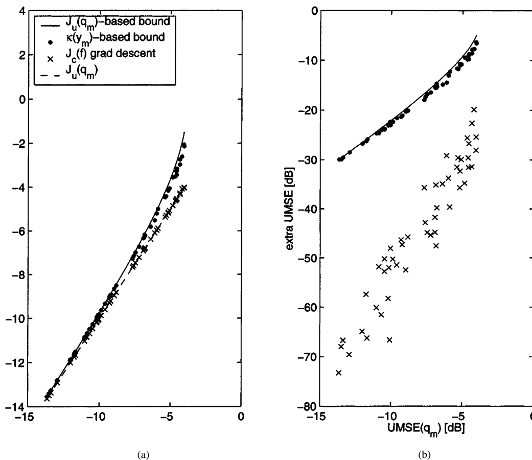
Fig. 6. Bounds on CM-UMSE for N_f = 8, 10 BPSK sources, AWGN at -20 dB, and random \mathcal{H} .
