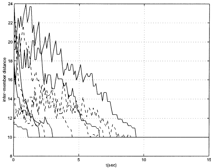
Fig. 8. Intermember distances of communicating neighbors in Fig. 7 during the convergence process.
