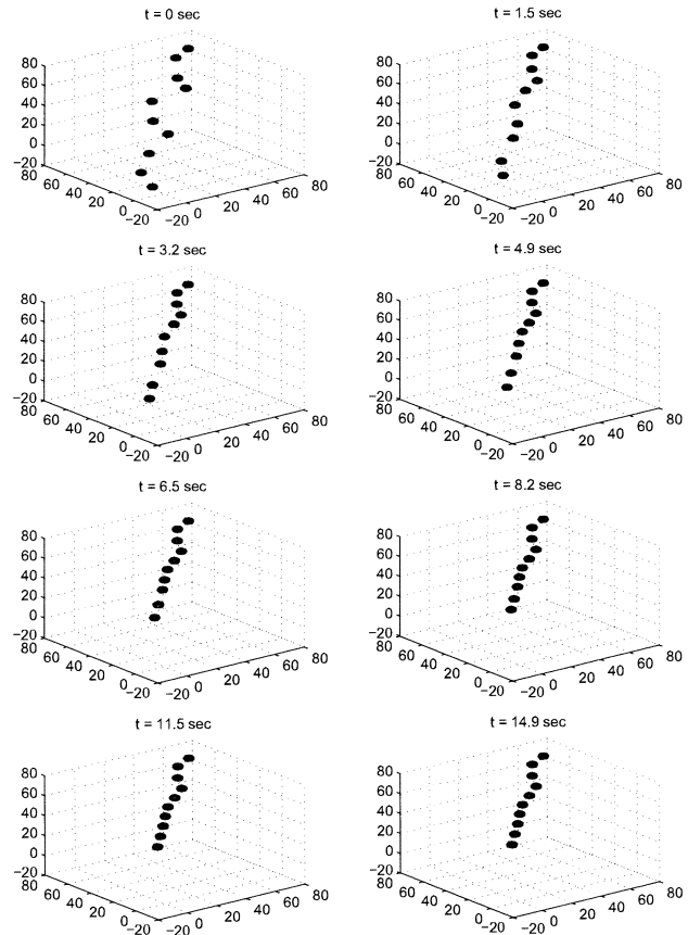
Fig. 7. Simulation of M = 3 -dimensional asynchronous ten-member asynchronous swarm with a fixed communication topology converging behavior.
