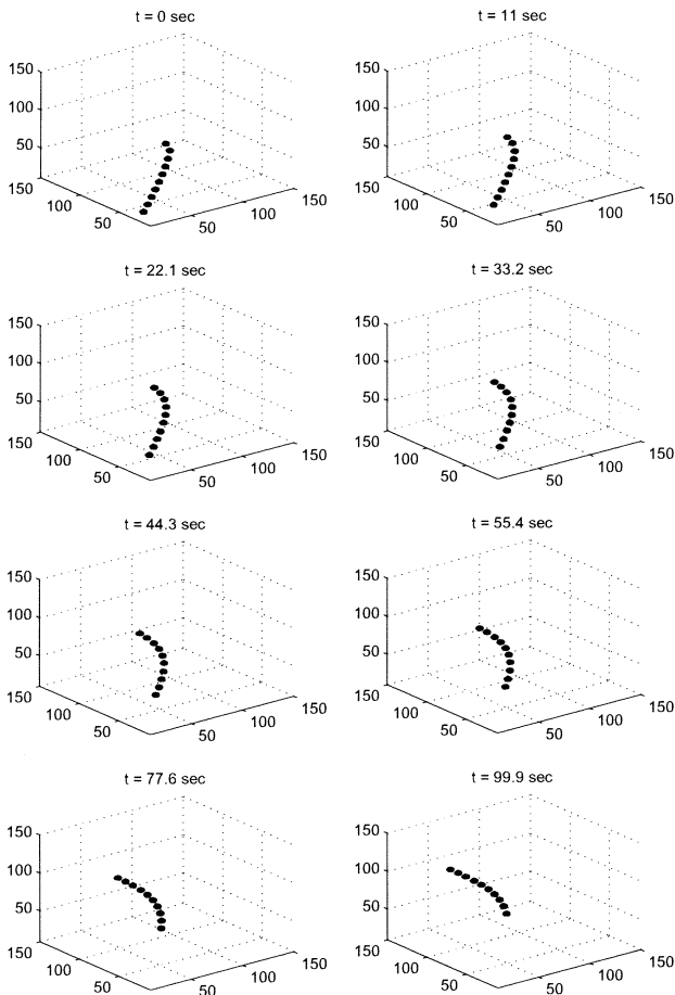
Fig. 9. Simulation of M = 3 -dimensional asynchronous ten-member asynchronous mobile swarm with a fixed communication topology following an edge-leader.
