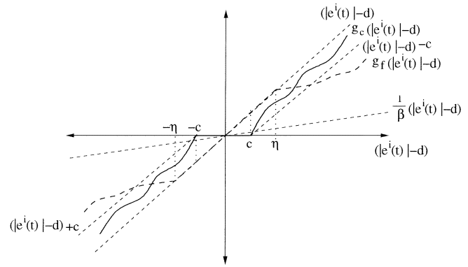
Fig. 6. Function g_c(e^i(t) - d) (solid) and g_f(e^i(t) - d) (dashed).
